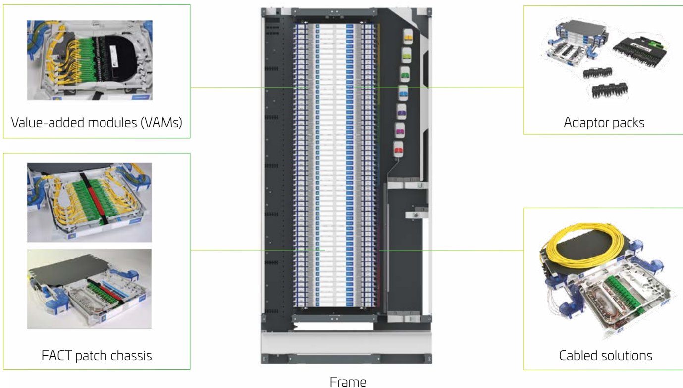
Figure 3: Cross-connect frame breakout with standard building blocks
