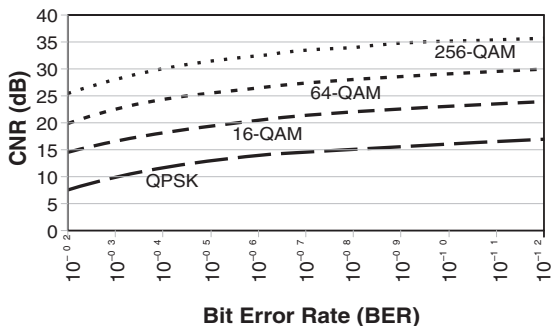
CNR in Relation to BER
