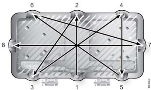
8 Bolt Tightening Sequence
