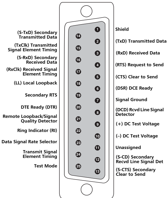
EIA-232 DB25 Female Connector
